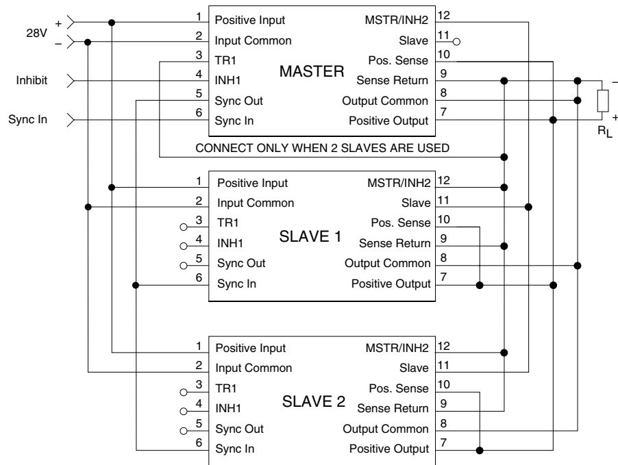
FIGURE 2: PARALLEL CONNECTIONS
